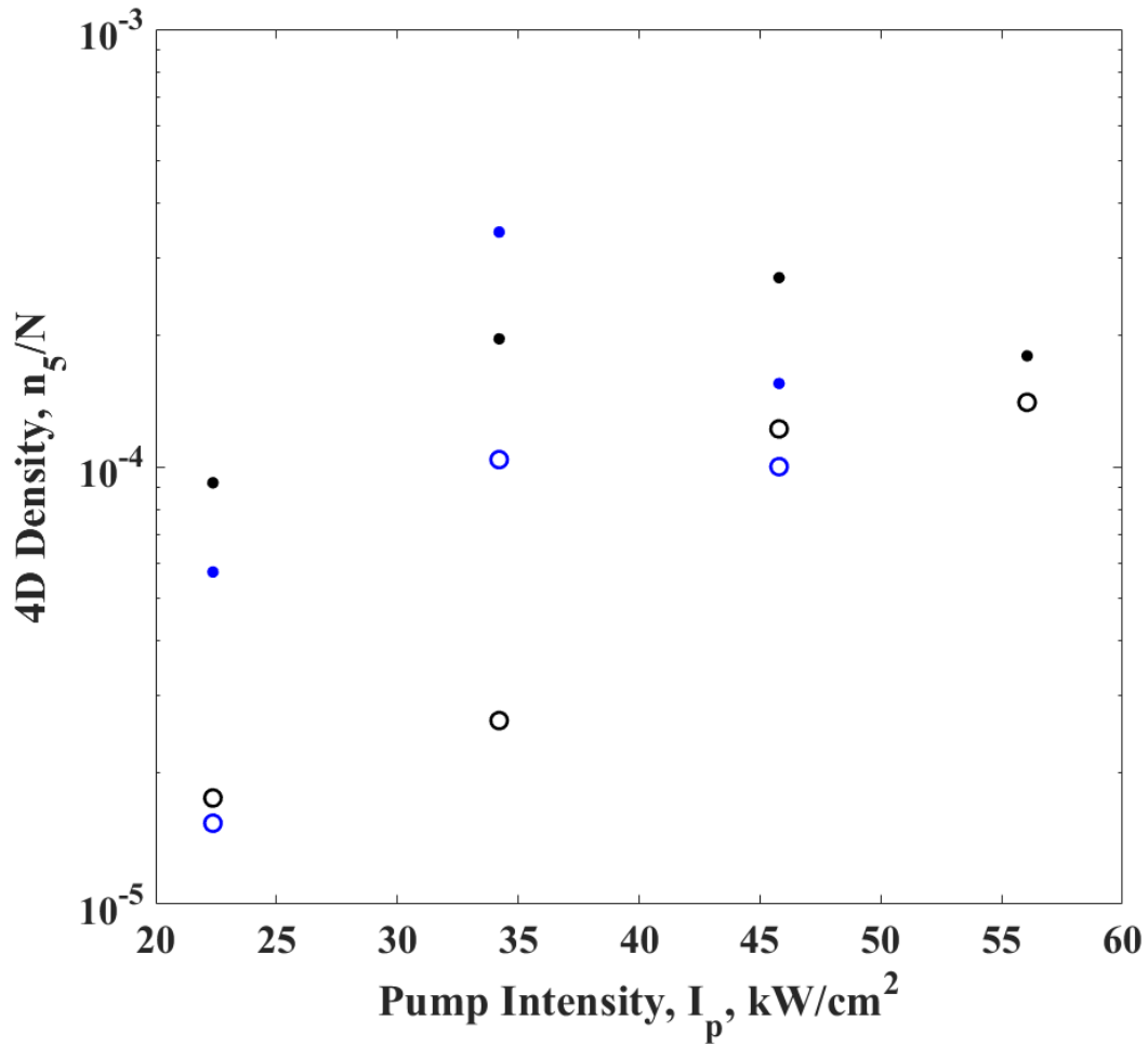
Figure 47. The observed (●) and predicted (○) density in the 4^2D state as a function of pump intensity at N \sim 2 \times 10^{13} \text{ cm}^{-3} with helium pressures of P=450 (black) and 850 (blue) Torr. The model presented in (80) is used to calculate the intermediate prediction.
