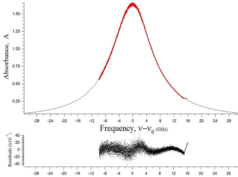
Figure 19. An example K 4^2S_{1/2} - 5^2P_{3/2} diagnostic with K density of N = 0.65 \times 10^{14} \text{ cm}^{-3} at bed temperature of T = 473 \text{ K} ; red points represent the observed spectra, and the black curve is the Lorentzian fit.
