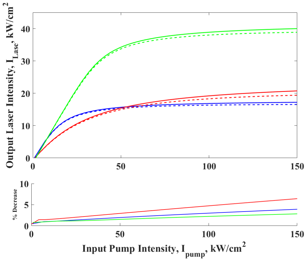
Figure 16. Laser intensity as a function of pump intensity, with and without multi-level kinetics (---). The cases presented here are the same as in fig:PsiOmega. The blue is consistent with the parameters in Table 3, the alkali density is doubled for the green and the helium density is doubled for the red.
