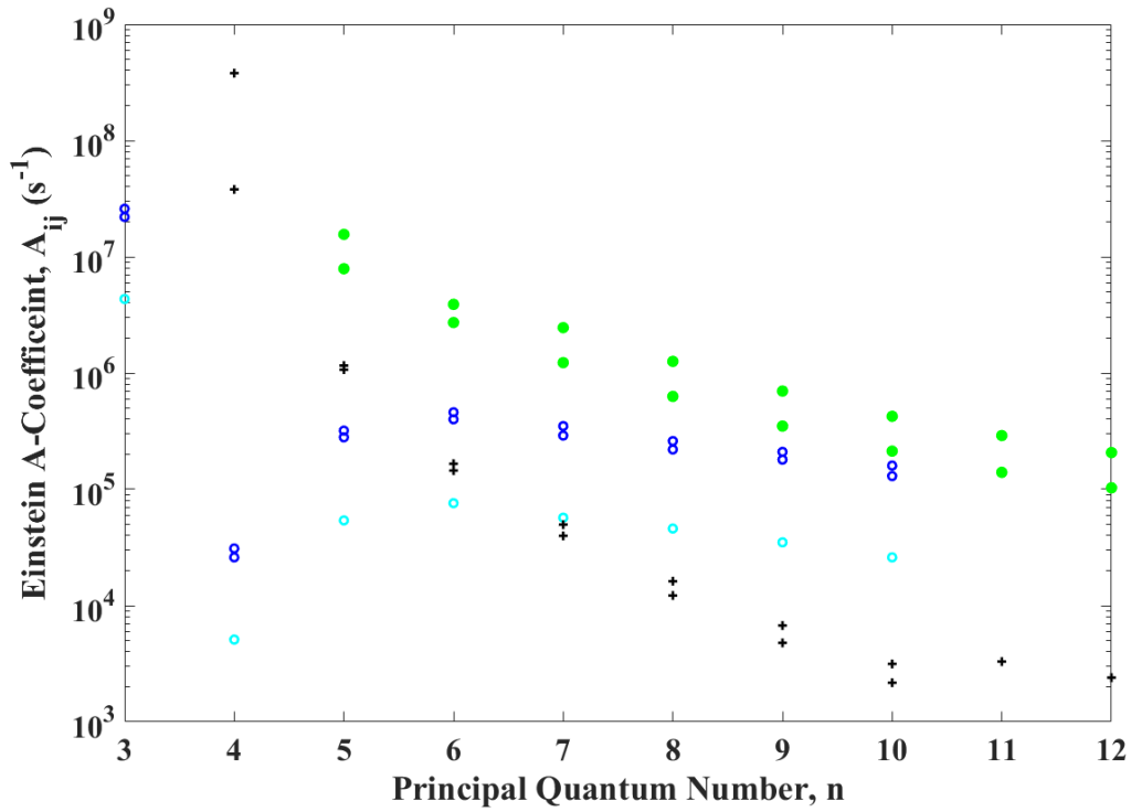
Figure 7. The Einstein A-coefficient for transitions in potassium as a function of the quantum number of the initiating state. Each trend is a different transition type; (green ●) S_{\frac{1}{2}} \rightarrow P_{\frac{3}{2}, \frac{1}{2}} , D \rightarrow P (dark blue ○: D_{\frac{3}{2}} \rightarrow P_{\frac{3}{2}, \frac{1}{2}} and light blue ○: D_{\frac{5}{2}} \rightarrow P_{\frac{3}{2}} ), and (black +) P_{\frac{3}{2}, \frac{1}{2}} \rightarrow S_{\frac{1}{2}} .
